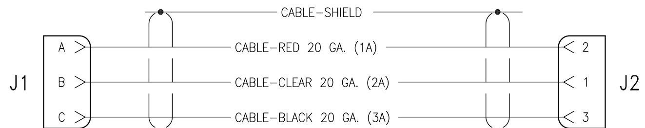
WIRING DIAGRAM
